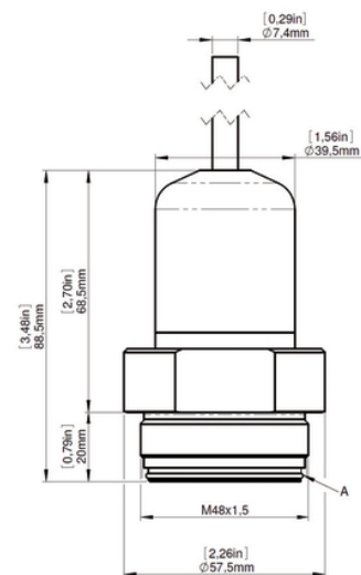
Flange version
